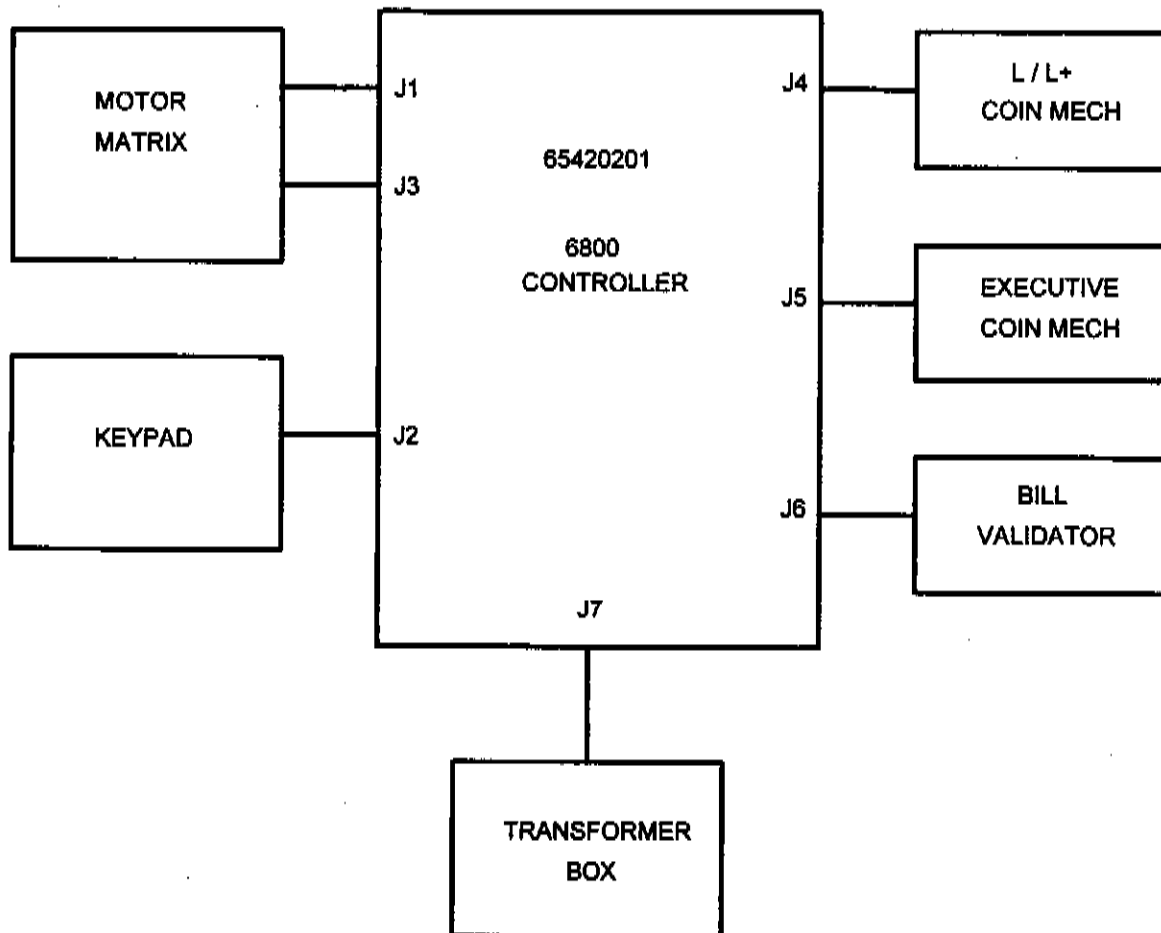
Figure 4-2. Block Diagram
