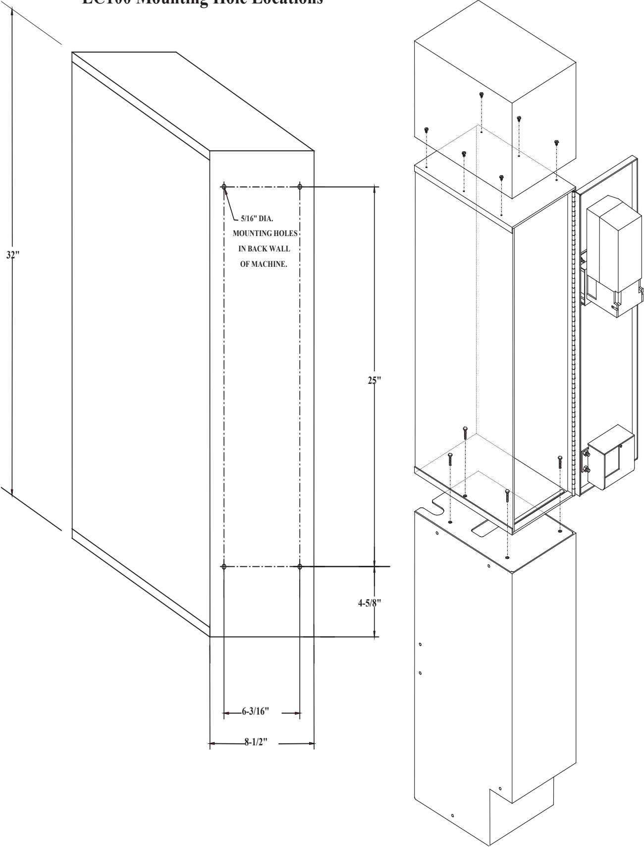
EC100 Mounting Hole Locations
